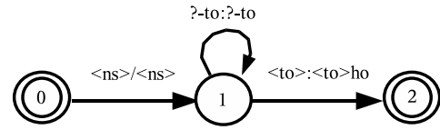
Fig. 4. TFFST model for the obligation in Rule 1 ( ns is NetworkSelected , to is TimerOver , and ho is handoff )
