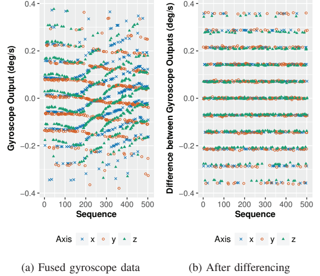
Fig. 4: Gyroscope data collected via JavaScript (iPad Air)
