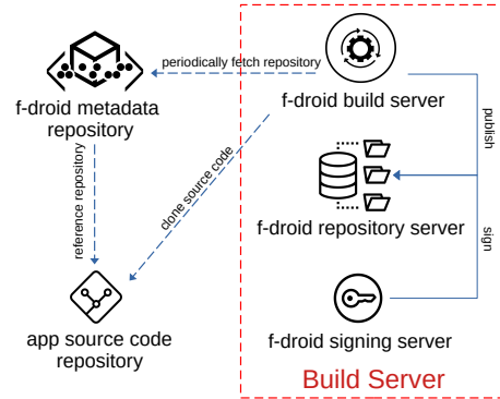
Fig. 4: Build server
