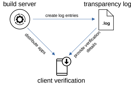
Fig. 3: System overview
