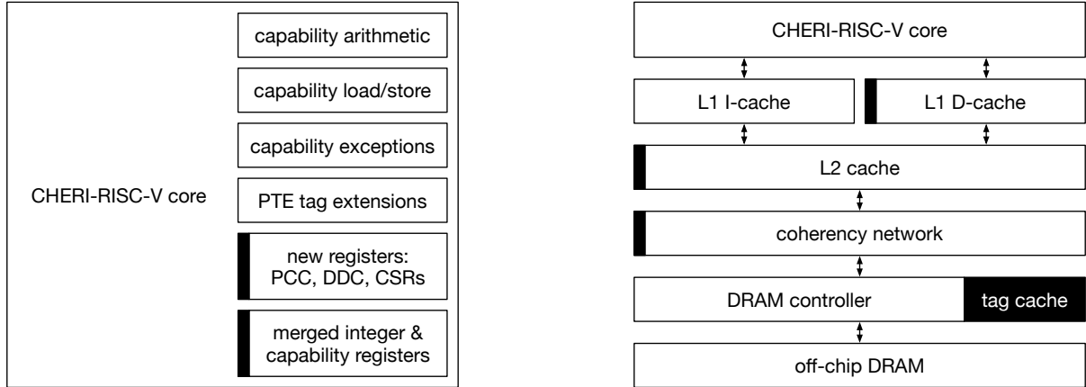
Figure 3.1: CHERI-RISC-V extensions to a processor core and memory hierarchy.
